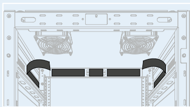
vent blockers magnetized on one side only to eliminate stray magnetic fields
