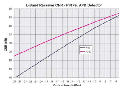
Adv. L-Band Rx CNR with PIN & APD
