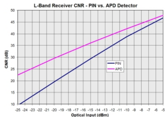
Advanced L-Band Rx CNR with PIN & APD
