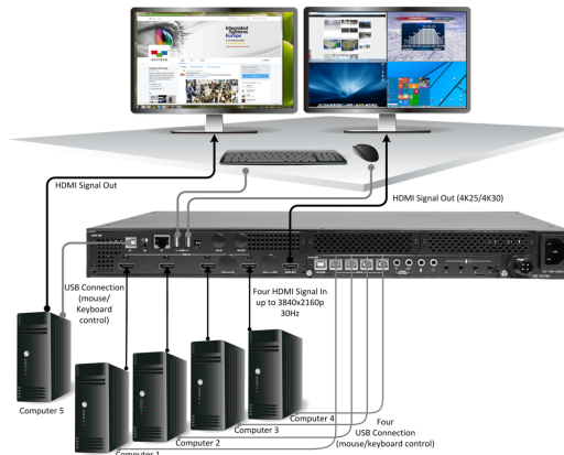
QuadraVista KVM UHD with dual-head workstation
