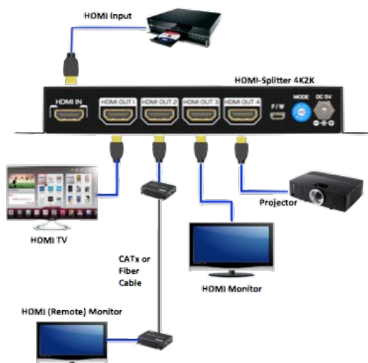
VideoSplitter HDMI 4K60 with extended video
