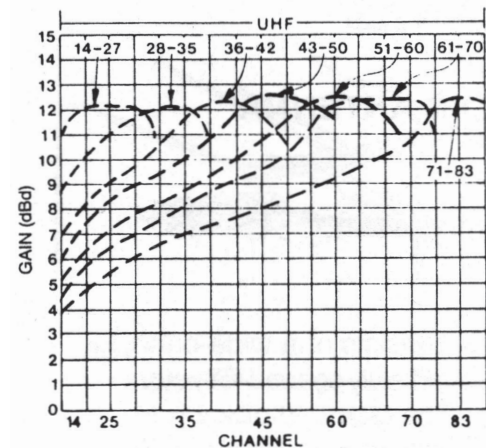
J-275D-K-* GAIN CURVES
