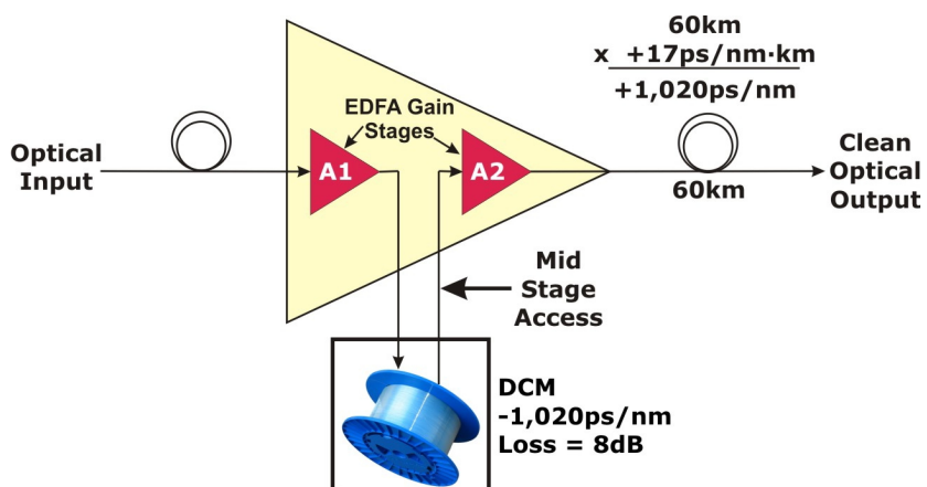
Figure 1 - Typical DCM Application
