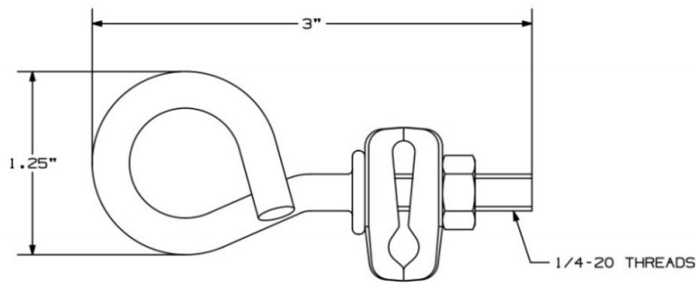
Q Span Clamp
