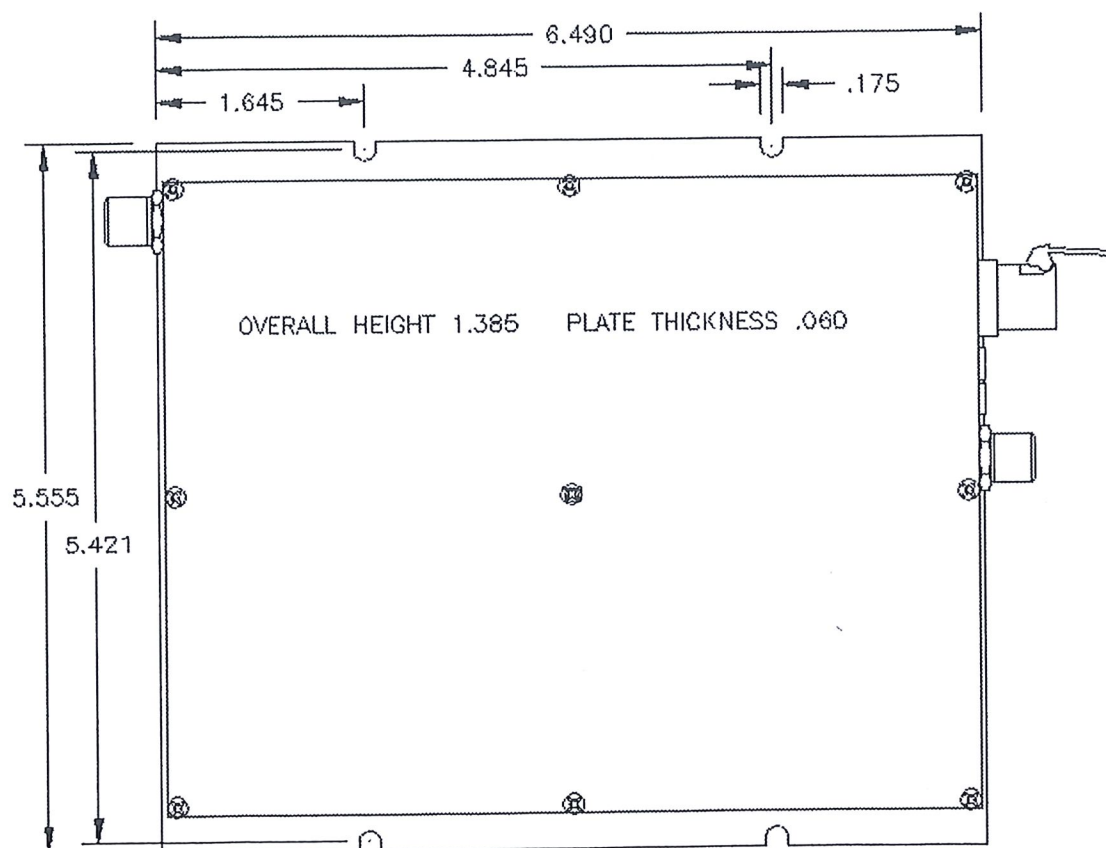
Figure 1 - OTOT-1220-xx Mounting Diagram
