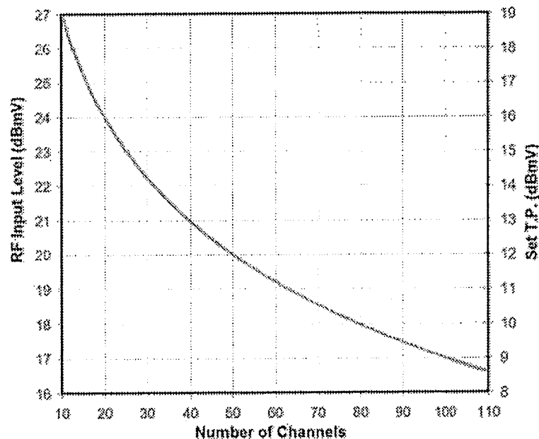
Figure 2 - Input Level vs. Channel Loading - Low-Power Units
