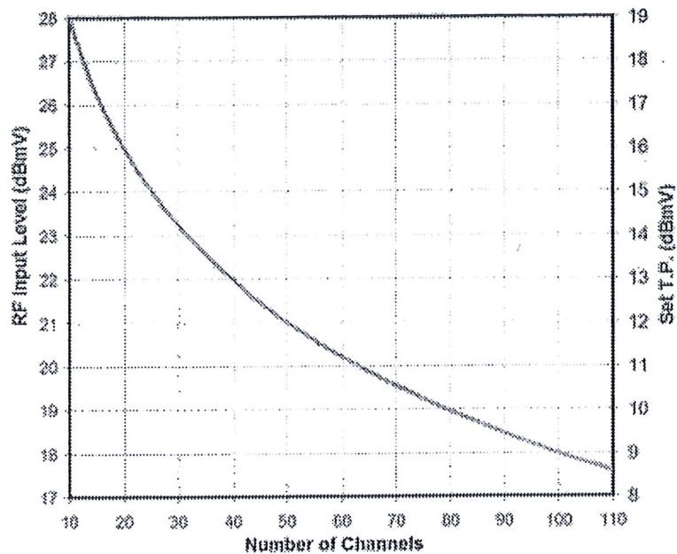
Figure 3 - Input Level vs. Channel Loading - High-Power Units
